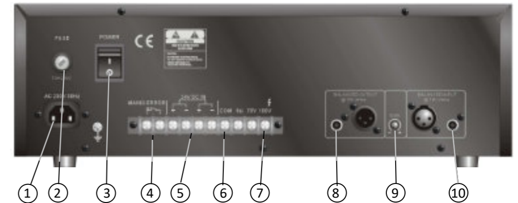
SINUS 40 amplifier / similar to SINUS 20/10 amplifier
