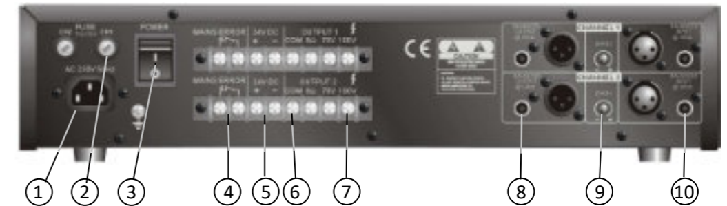
SINUS 40 amplifier / similar to SINUS 20/10 amplifier
